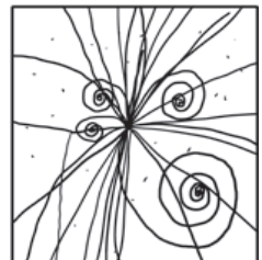
HIGGS BOSON
